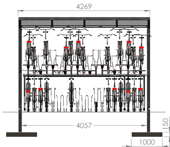
T-Hide Up double-sided 1 section - h.2.h. 400 mm
