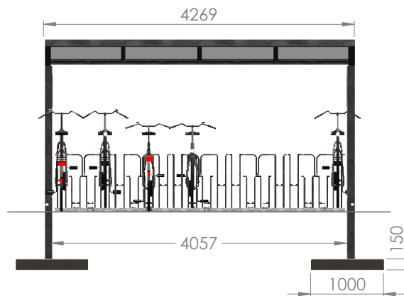
T-Hide double-sided 1 section - h.2.h. 400 mm
